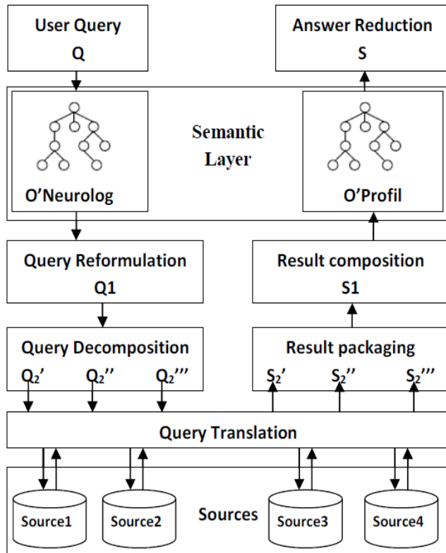
Figure 2. Process Query
