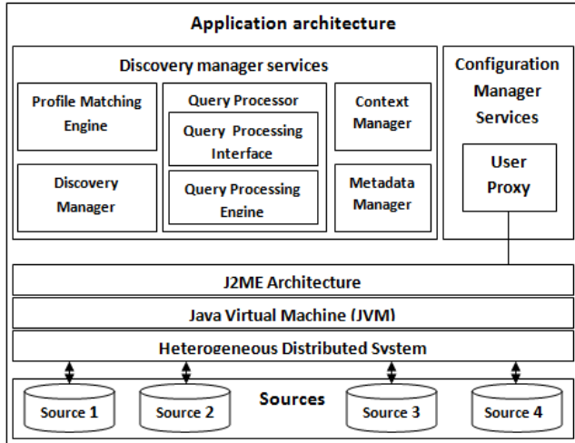
Figure 1. Application architecture
