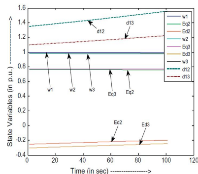
Fig 6. State space parameters in time domain (abnormal situation).
