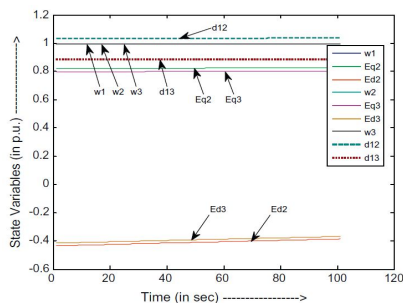
Fig.5. State space parameters time domain (Normal situation).
