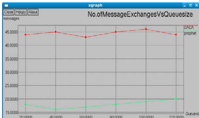
Fig. 3 No of Message Exchanges Vs Queue Size
