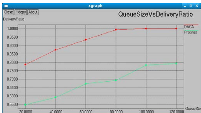
Fig. 1 Queue size Vs Delivery Ratio
