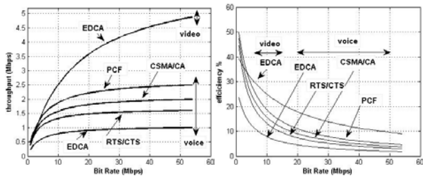
Fig.13 Throughput 802.11e
